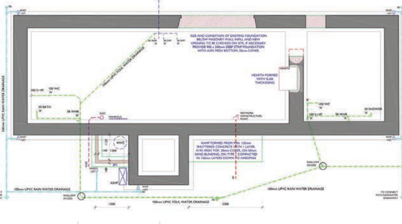
FOUNDATION PLAN SCALE 1:50
