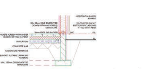
SOLUM DETAIL SCALE 1:20
