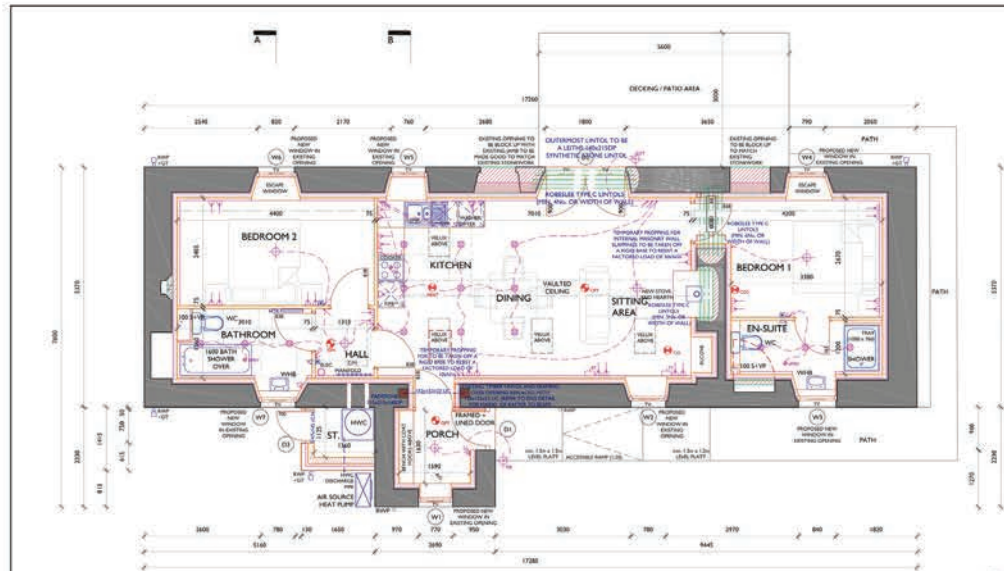
GROUND FLOOR PLAN SCALE 1:50
